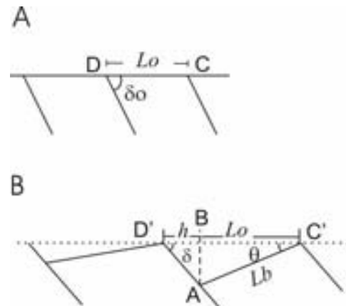
FIGURE 8 | Sketch to illustrate the relationships among parameters for a domino faults assuming vertical shear (Westaway and Kuszniir, 1993).
