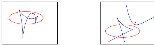
FIGURE 2. All possible configuration for the point–ellipse bisector (in blue).
